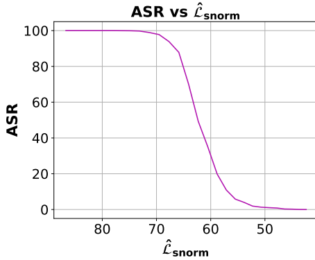
Figure 4: Effect of spectral norm minimization on ASR.
